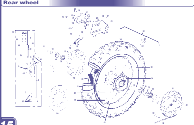
Rueda trasera / Rear wheel GASCAS EC 2003
