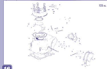
Cilindro - Culata - V. Escape / Cylinder - Cyl. head GASGAS EC 2003
