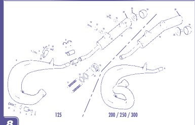
Tubo escape / Exhaust GASGAS EC 2003
