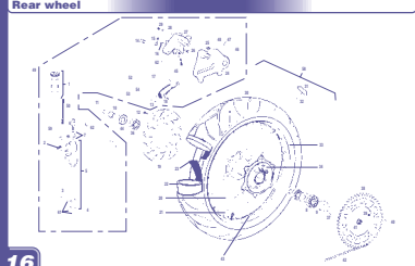
Rueda trasera / Rear wheel GASCAS SM 2002
