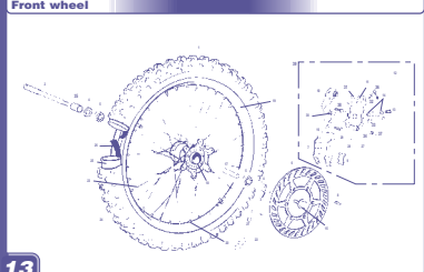
Rueda delantera / Front wheel GASCAS EC 2003
